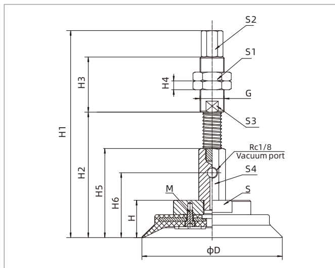
SH40-125 Lateral direction
