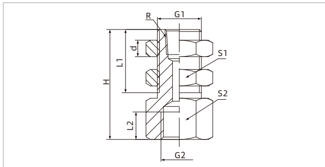
Vertical female thread
