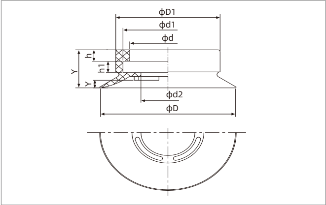
SPU30-100 ◇ Note: The dimensional tolerance conforms to GBT 3672.1-2002-1 M3 rubber product dimensional tolerance standard
