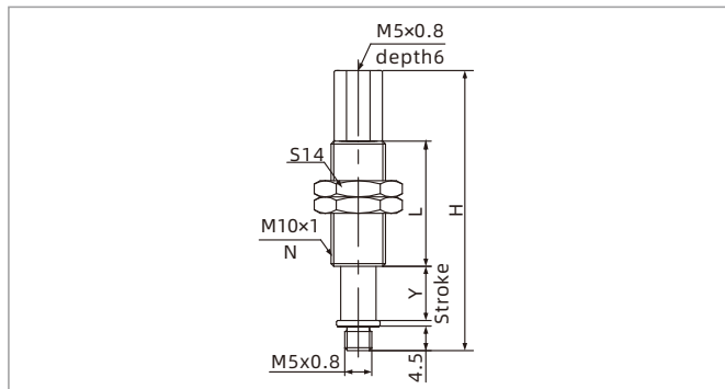
M5M-Vertical male thread connection
