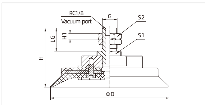
SH40-125 Vertical, male thread connection
