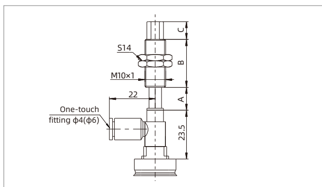
Lateral-One-touch fitting
