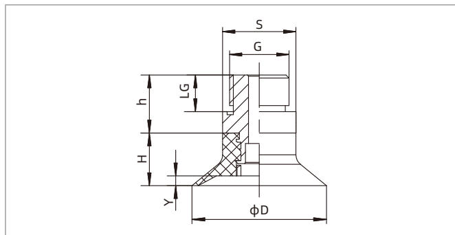
SFP20-40 Male thread connection
