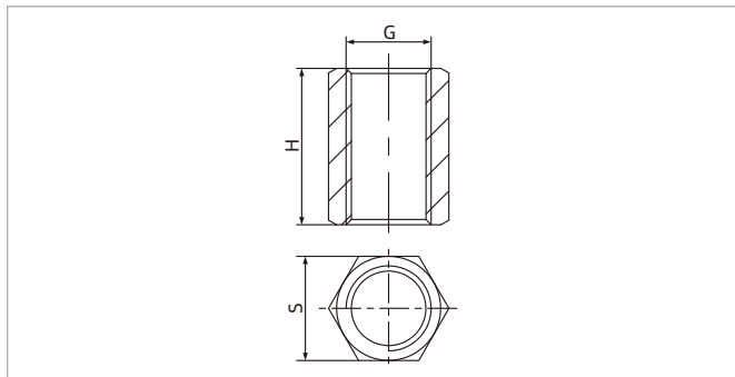
Equal diameter female-female thread
