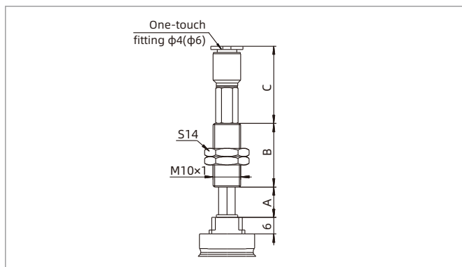
Vertical-One-touch fitting
