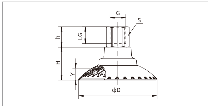
F - Female thread connection
