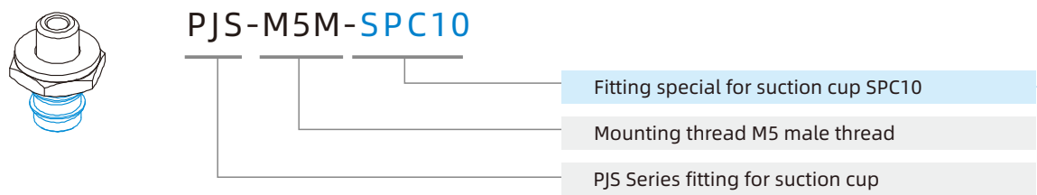
PJS series fitting for suction cup
