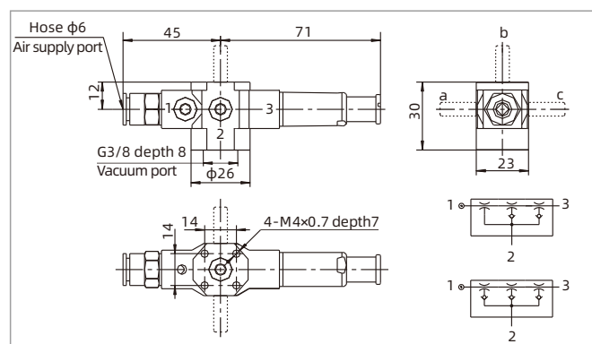
C for AGS-N series
