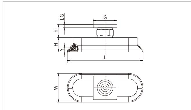
RA-Rectangular adapter
