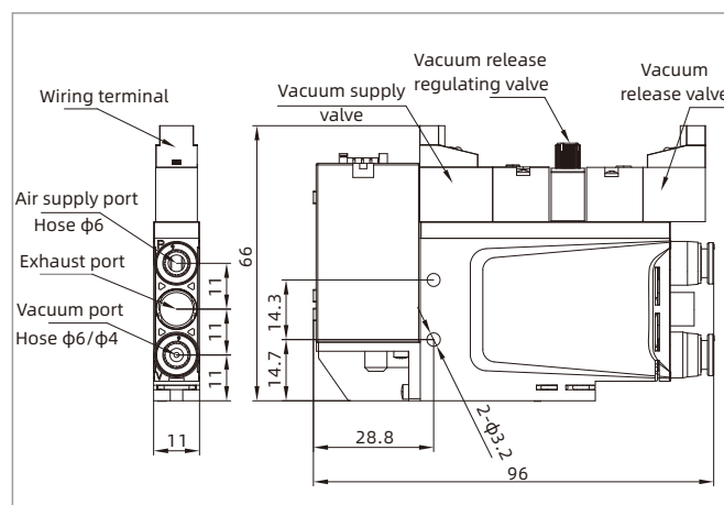
AZQ-□-□ Single body of vacuum generator type
