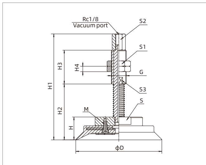
SH40-125 Vertical direction
