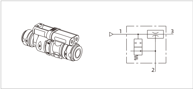
ABP-10 Note: 1. Air supply port, 2. Vacuum port, 3. Exhaust port
