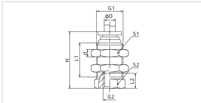
Vertical one-touch fitting
