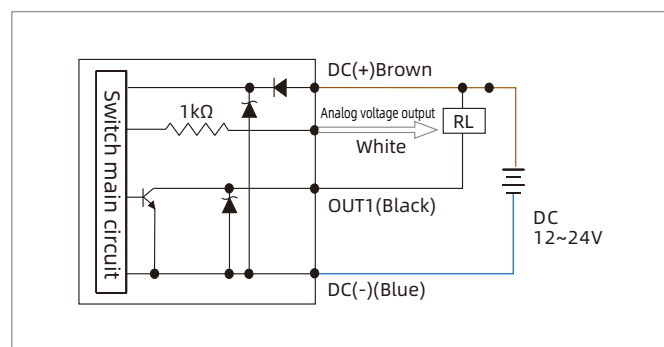
ZPDT-CNV-R1M 1PNP+Analog voltage output(1-5V)
