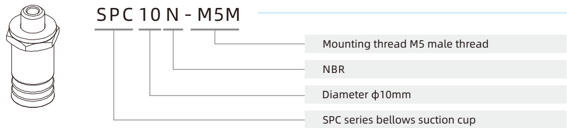
Suction cup + PJS series fitting for suction cup
